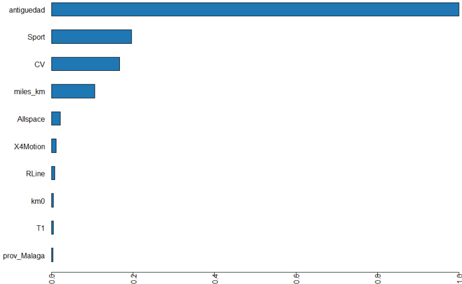
Variable Importance: GBM
